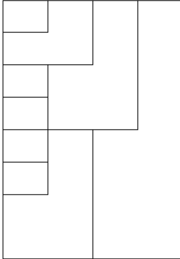
Figure 4: The split-radix transform has L-shaped butterflies
