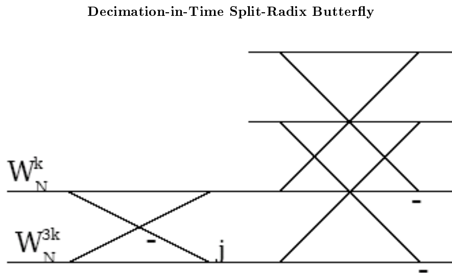
Figure 3: The split-radix butterfly mixes radix-2 and radix-4 decompositions and is L-shaped
