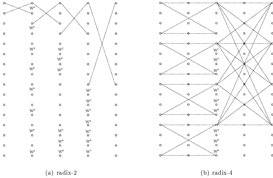
Figure 1: See Decimation-in-Time (DIT) Radix-2 FFT 8 and Radix-4 FFT Algorithms 9 for more information on these algorithms.
