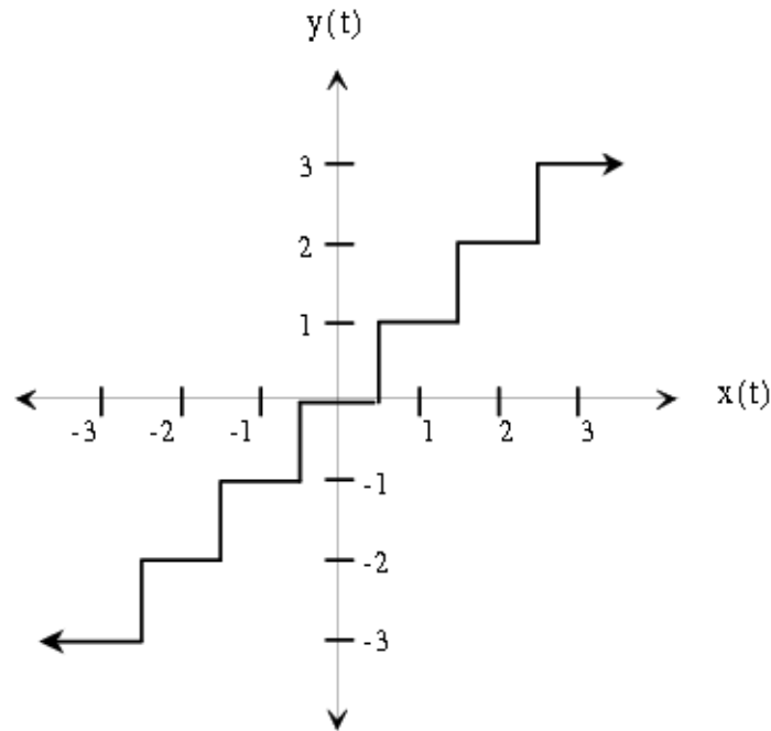
Figure 1: Input-output relation for a 7-level uniform quantizer.
