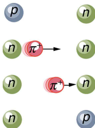
Figure 1: The strong nuclear force is transmitted between a proton and neutron by the creation and exchange of a pion. The pion is created through a temporary violation of conservation of mass-energy and travels from the proton to the neutron and is recaptured. It is not directly observable and is called a virtual particle. Note that the proton and neutron change identity in the process. The range of the force is limited by the fact that the pion can only exist for the short time allowed by the Heisenberg uncertainty principle. Yukawa used the finite range of the strong nuclear force to estimate the mass of the pion; the shorter the range, the larger the mass of the carrier particle.
