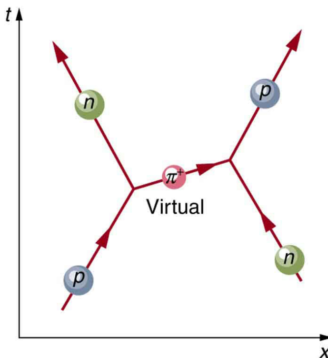
Figure 3: The image shows a Feynman diagram for the exchange of a \pi^+ between a proton and a neutron, carrying the strong nuclear force between them. This diagram represents the situation shown more pictorially in Figure 1.
