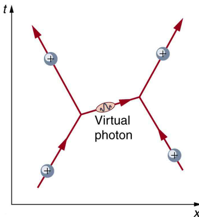
Figure 2: The Feynman diagram for the exchange of a virtual photon between two positive charges illustrates how the electromagnetic force is transmitted on a quantum mechanical scale. Time is graphed vertically while the distance is graphed horizontally. The two positive charges are seen to be repelled by the photon exchange.
