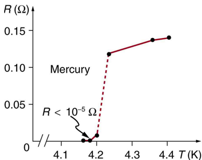
Figure 1: A graph of resistivity versus temperature for a superconductor shows a sharp transition to zero at the critical temperature T_c . High temperature superconductors have verifiable T_c s greater than 125 K, well above the easily achieved 77-K temperature of liquid nitrogen.
